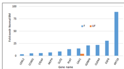
Fig 5. Expression of DTC associated transcripts in filtered and unfiltered BM specimens.
