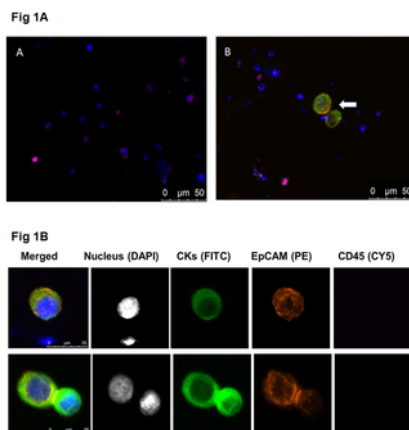
Fig 1. Images of the filter-captured breast cancer tissue culture cells.
