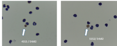
Fig 4. RNA-In situ hybridization for ERBB2 gene expression.
