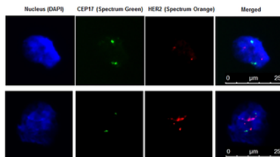
Fig 3. Her2-FISH analysis of DTCs from breast cancer patient BM.
